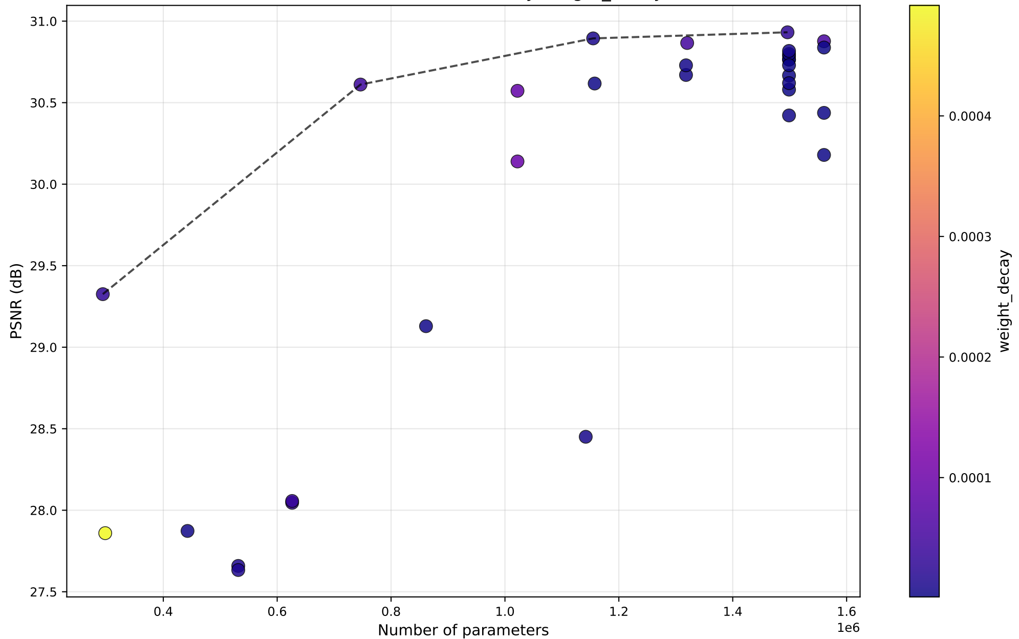
PSNR vs #Params — DAT — by weight_decay
